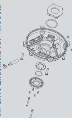
Non-drive Endshield Kit - W3Seal
