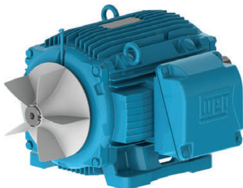
Figure 19 - Cooling system.
