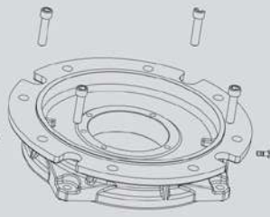
Non-drive Endshield Kit - W3Seal
