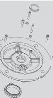
FF Flange Kit
