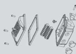
Auxiliar Terminal Box Kit
