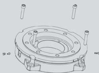
Drive endshield Kit - W3Seal
