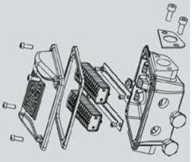
Auxiliar Terminal Box Kit
