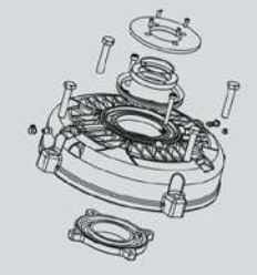
Drive endshield Kit - W3Seal
